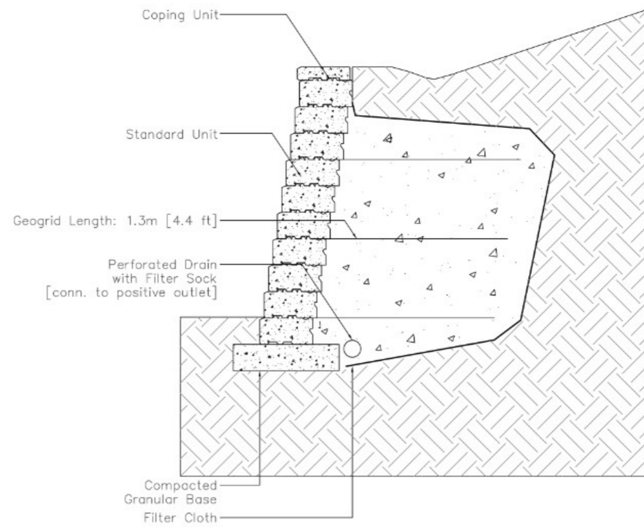
SECTION—GEOGRID REINFORCED RETAINING WALL SCALE: NONE
