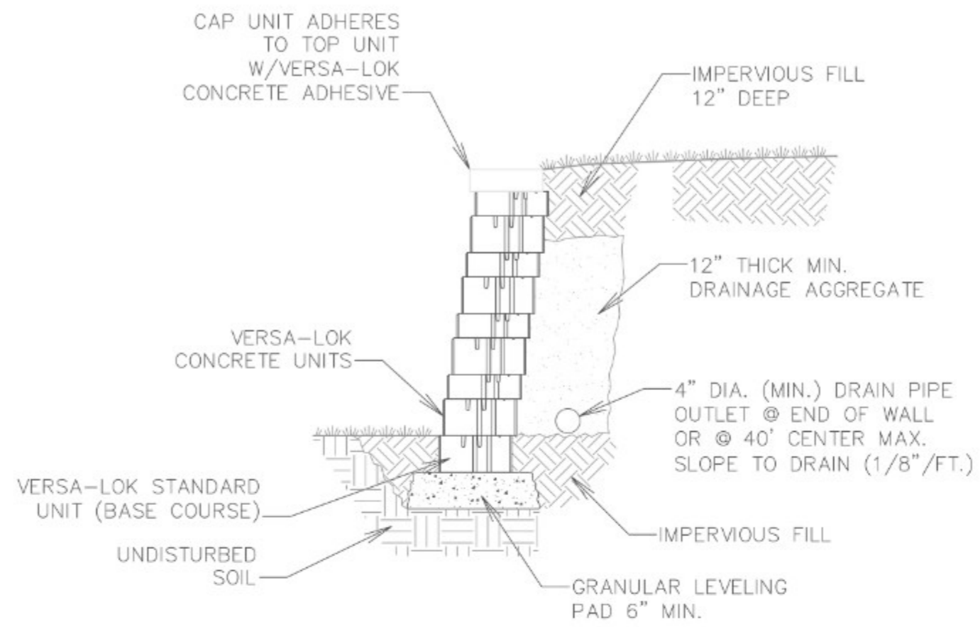
SECTION—UNREINFORCED RETAINING WALL SCALE: NONE
