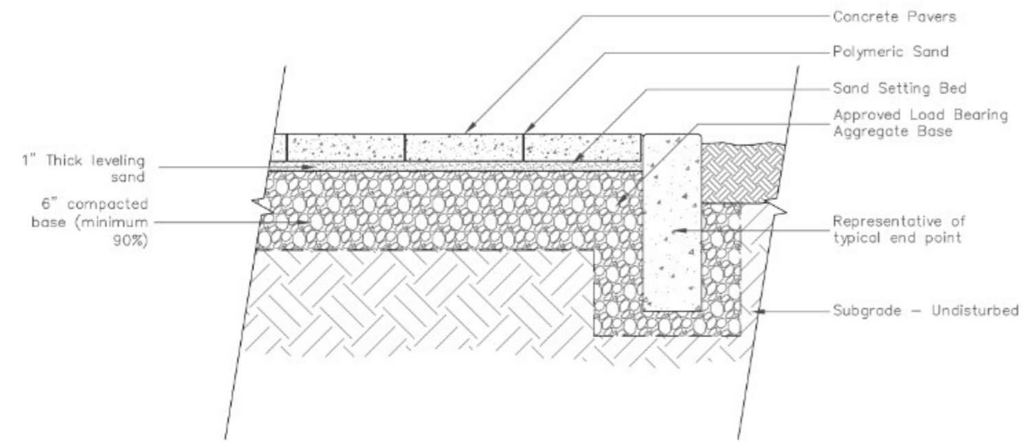
SECTION—CONCRETE PAVER INSTALLATION SCALE: NONE
